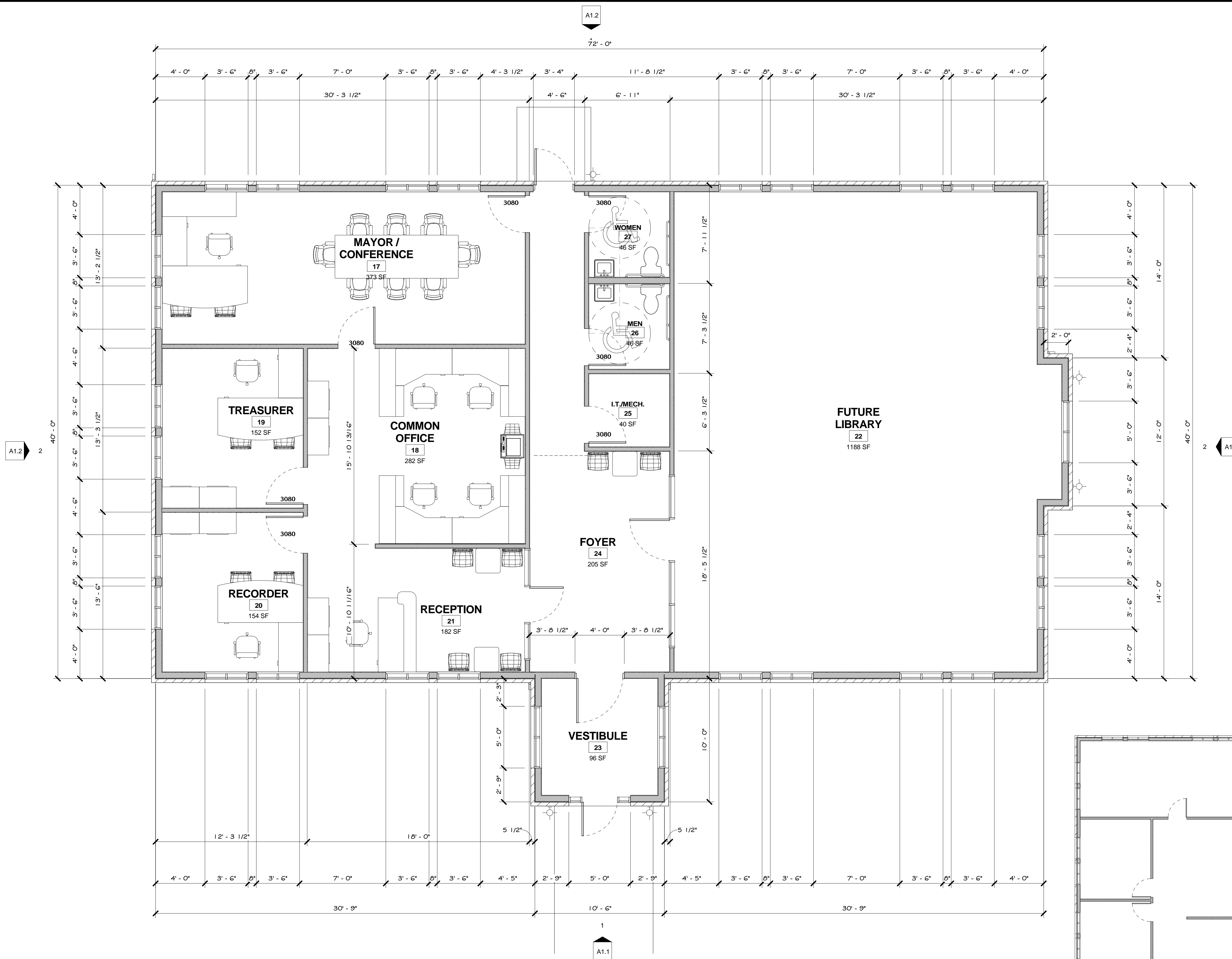
First Floor 1/4" = 1'-0"
